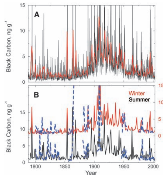
Fig. 1. (A) Monthly (black) and annual (red) BC concentrations from 1788 through 2002 measured in the Greenland D4 ice core. (B) Winter and summer BC concentrations show that long-term changes in BC were greater in winter (red) than in summer (black) during the late 19th and early 20th centuries. Winter and summer BC concentrations measured in the D5 ice core (6), located \sim 350 \text{ km} south of the D4 site (blue dashed trace), indicate that observed BC changes were at least regional in extent. The maximum monthly BC value of 58.8 \text{ ng g}^{-1} occurred in summer 1854.
