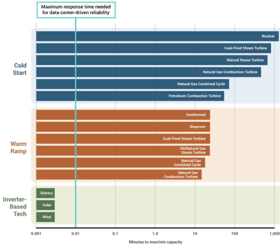
Figure 8: Minutes Needed for a Power Plant to Reach Max/Min Capacity
