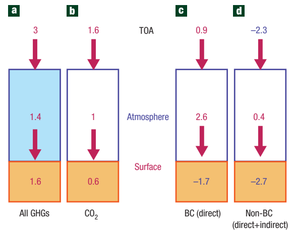
Figure 2 Comparison of the global mean radiative forcing due to greenhouse gases (GHGs) with that of ABCs. a,b , Forcing for all GHGs ( \text{CO}_2 , \text{CH}_4 , \text{N}_2\text{O} , halons and ozone) ( a ), and for \text{CO}_2 ( b ). The number at the top of the atmosphere box (blue box) is the top-of-the atmosphere (TOA) forcing; the number within the atmosphere box is the atmospheric forcing; and the number within the brown box is the forcing at the surface. The forcing values represent the change in radiative forcing due to increase in gases for the year 2005, which is the same as the forcing from pre-industrial to present. The TOA numbers are taken from ref. 68 and the atmospheric and surface forcings are derived from an atmospheric radiative transfer model. The numbers at the surface and the atmosphere are slightly adjusted to agree with the TOA IPCC forcing. The uncertainty in the forcing values is \pm 20\% . c , BC forcing obtained by running the Chung et al. analysis 23 with and without BC. The forcing values are valid for the 2001–2003 period and have an uncertainty of \pm 50\% . d , Non-BC forcing. This includes the direct and the indirect forcing. The direct forcing is obtained by subtracting the total anthropogenic forcing in Chung et al. from the BC forcing shown in b . The indirect forcing (of about 1 \text{ W m}^{-2} at the TOA and at the surface) is an average of values derived from recent studies 35–37 .
